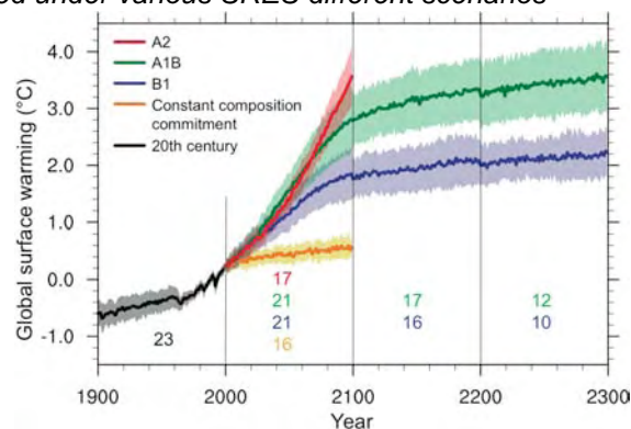
Figure 1 Mean global temperature evolution according to the multiple GCM output grouped under various SRES different scenarios
